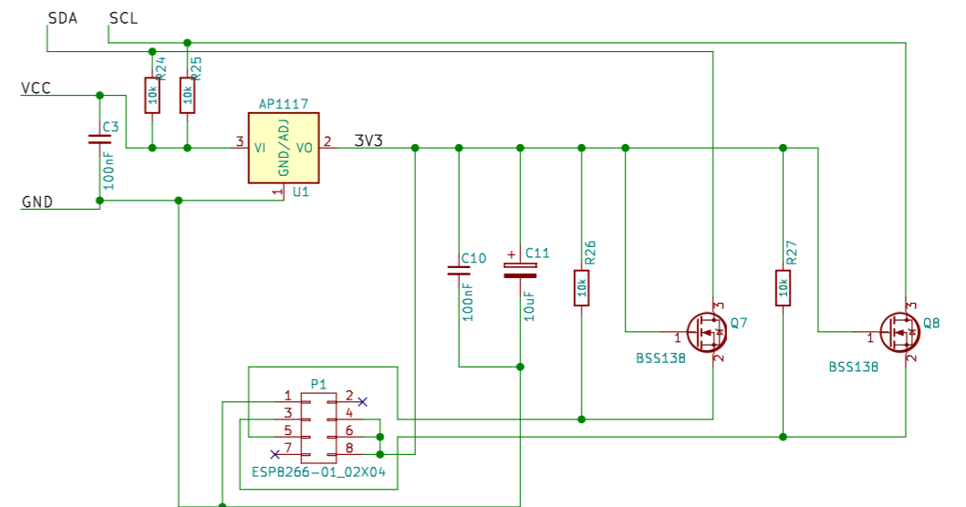
ESP8266 Regulator and I2C level shifter
